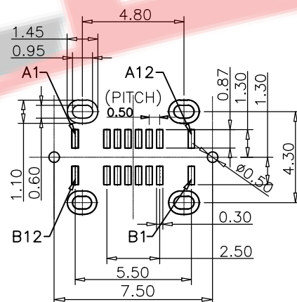
RECOMMENDED P.C.B. LAYOUT TOLERANCE UNSPECIFIED \pm 0.05\text{mm}
