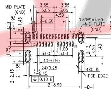
RECOMMENDED PCB LAYOUT (TOLERANCE: ±0.05)
