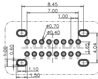
RECOMMEND P.C.B LAYOUT TOLERANCE UNSPECIFIED ±0.05mm
