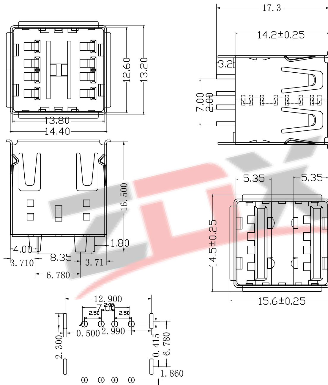
RBCOMMEND P.C.B. PATTERN LAYOUT
