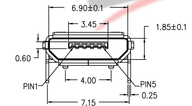
MICRO USB B TYPE PIN ASSIGNMENTS
