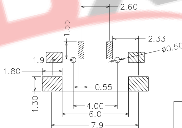
RECOMMENDE.P.C.B LAYOUT(TOP VIEW) EFAULT YOLERANCE:±0.05
