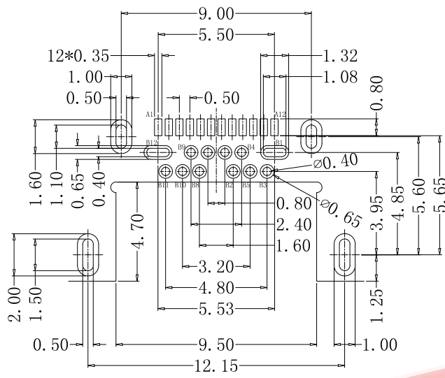
RECOMMENDED PCB LAYOUT, TOP VIEW (THICKNESS=0.60MM; TOLERANCE: ±0.05)
