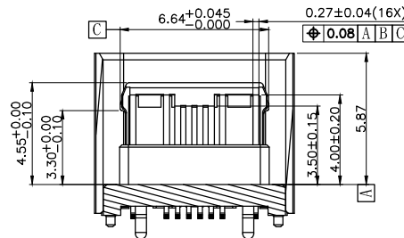
SECTION B-B SCALE 1:1
