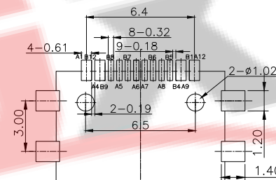
RECOMMENDED PCB LAYOUT Tolerance:±0.05mm
