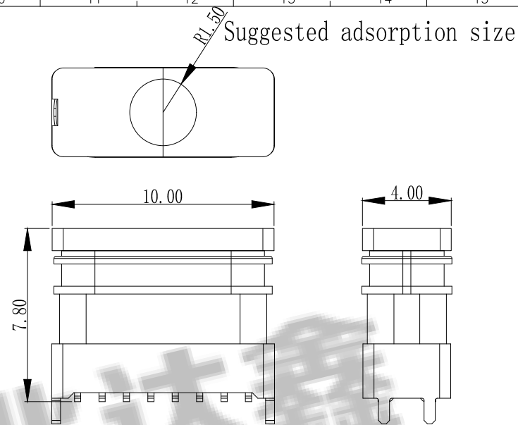
Install suction cap diagram
