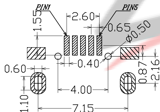
RECOMMENDED P.C.B LAYOUT (TOP VIEW) EFAULT YOLERANCE:±0.05
